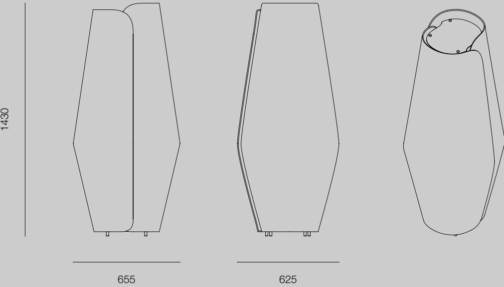
FLOOR XXL 1400 | FLOOR XXL 1400 OUTDOOR
