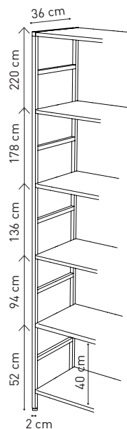
SPALLE Prof. 36 cm UPRIGHTS Depth 36 cm
