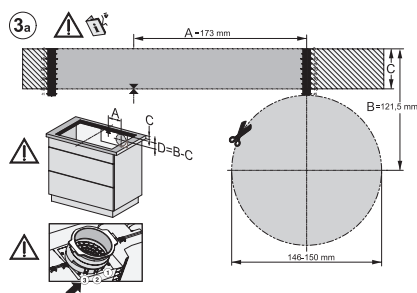
KMDA7272-1FL/FR, KMDA7473-1FL/FR, KMDA7272FL/FR, KMDA7473FL/FR – Installation variant 13 Circulating air
