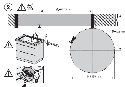
KMDA7272-1FL/FR, KMDA7473-1FL/FR, KMDA7272FL/FR, KMDA7473FL/FR – Installation variant 6 Circulating air
